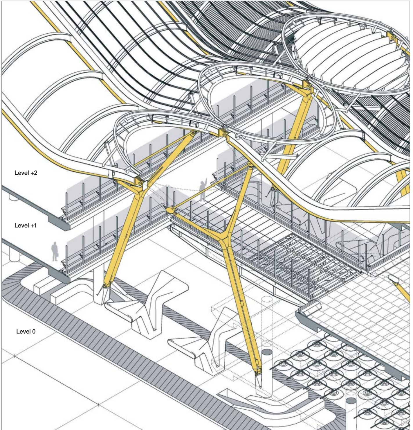
Terminal building 'B' canyon between check in and controls. Luggage collection at level 0 and horizontal connections
