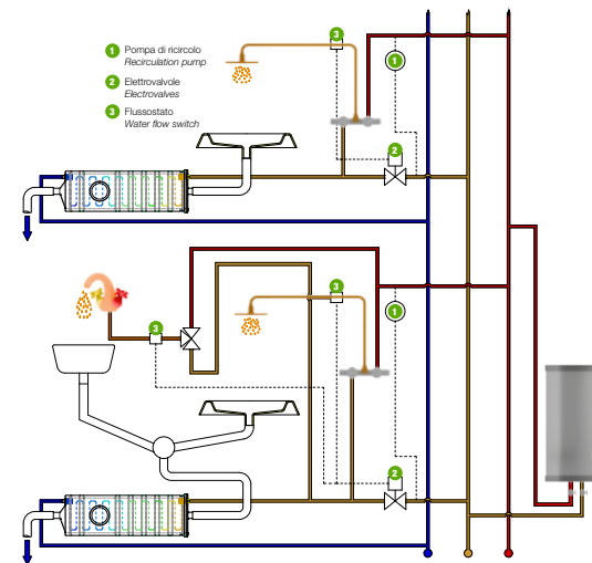
Collegamento multizona - Connecting multi-area Schema B recupero totale - Diagram B total recovery
