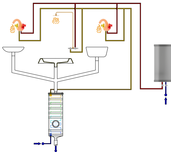
Collegamento monozona - Single-area connection Schema A - Diagram A
