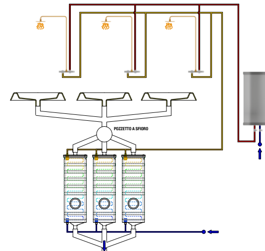
Collegamento parallelo - Parallel connection Schema A - Diagram A
