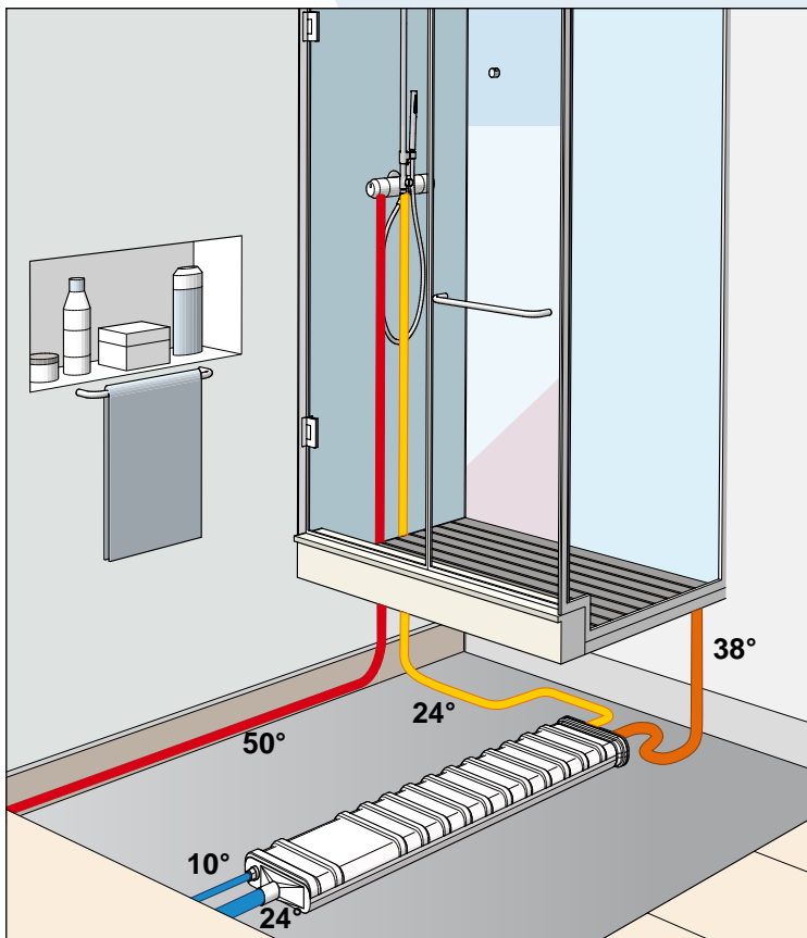
Schema applicativo A Application diagram A
