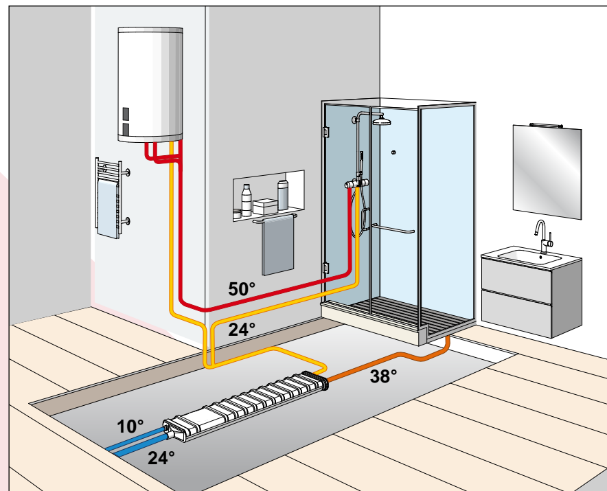
Schema applicativo B Application diagram B
