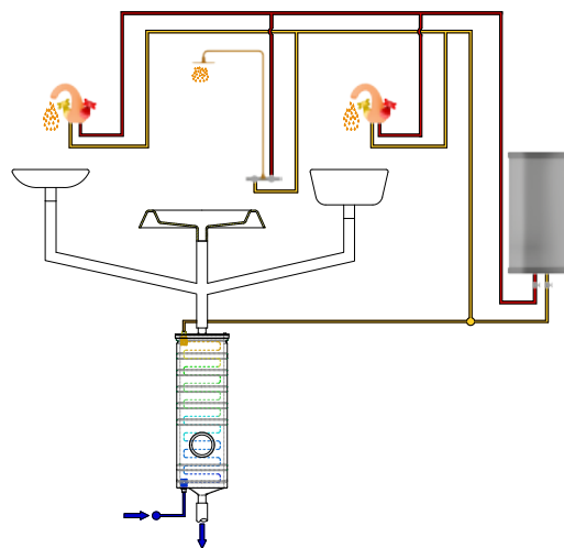
Collegamento monozona - Single-area connection Schema B recupero totale - Diagram B total recovery
