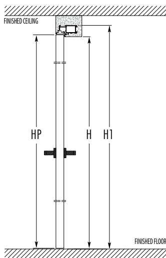
FRAME WITH HEADER
