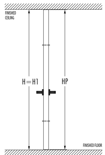
FRAME WITHOUT HEADER
