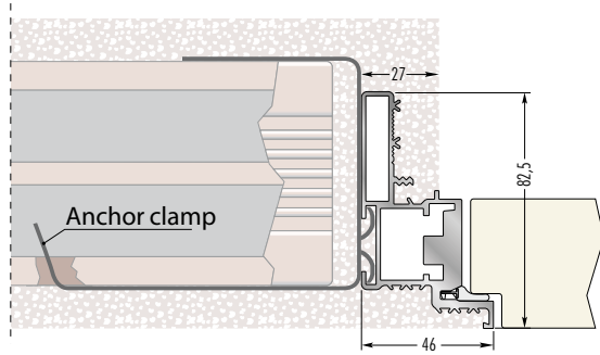
Frame on solid wall
