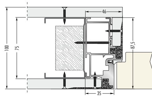
Frame on stud wall with one plate Finished wall thickness 100 mm
