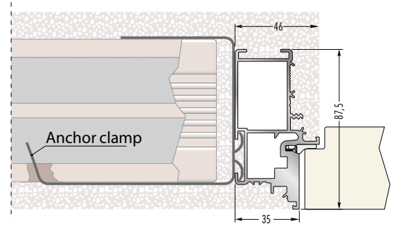
Frame on solid wall
