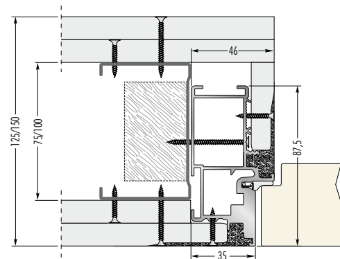
Frame on stud wall with three plates Finished wall thickness 125/150 mm
