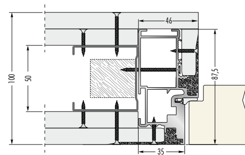
Frame on stud wall with two plates Finished wall thickness 100 mm
